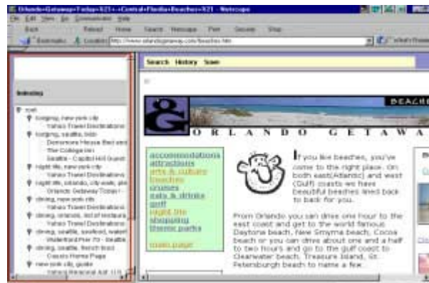
Figure 6. Screen Shot of Result of the “Index All” Function
